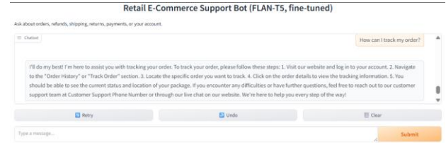
Fig. 7. The Gradio chat interface answering an order-tracking query with a structured, multi-step response.
