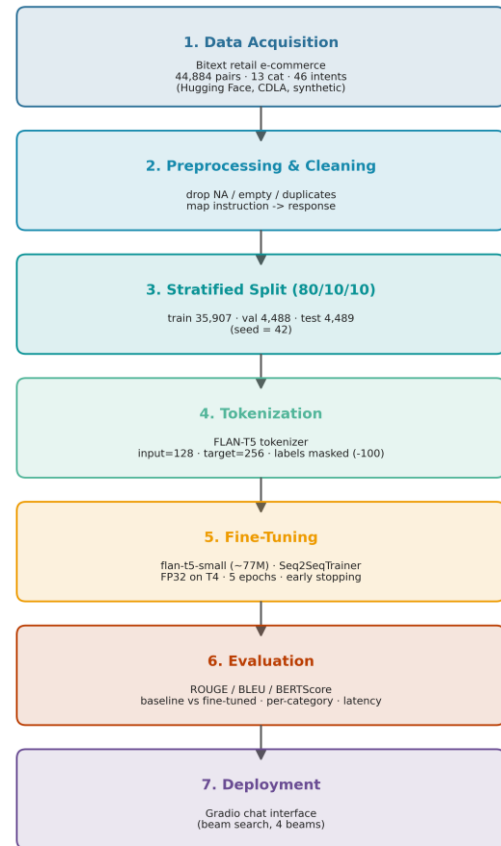
Fig. 8. End-to-end fine-tuning pipeline (data acquisition \rightarrow preprocessing \rightarrow stratified split \rightarrow tokenization \rightarrow fine-tuning \rightarrow evaluation \rightarrow deployment).
